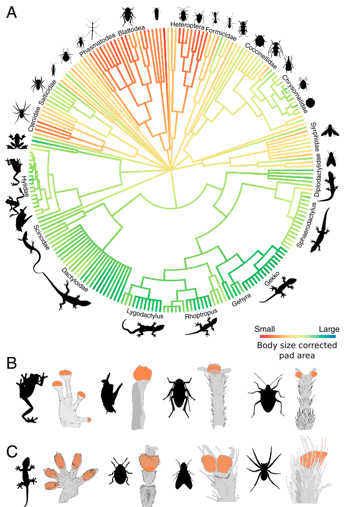
Fig. 3. (A) Overview of the diversity of taxa examined in this study. Branch lengths do not reflect time or base pair substitutions (see Materials and Methods ). Branches are colored according to a maximum likelihood estimate of the ancestral state of relative pad area (i.e., the residuals from a log-log regression of pad area against body weight), visualizing systematic differences in relative pad area between arthropods and vertebrates. All values apart from tip states are only approximate and are not used to support any conclusions (see Materials and Methods ). (B and C) Cartoons depicting footpad morphology for representative groups within the phylogeny shown above with smooth and hairy adhesive pads. Projected pad area is highlighted in orange for each representative (see Materials and Methods ).
